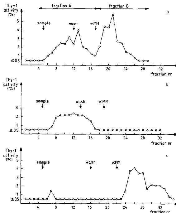
Fig.1. Affinity chromatography on lentil lectin–Sephacrose 4B: (a) thymocyte extract (3.5 ml sample); (b) pooled fraction A from expt a (4.5 ml sample); (c) pooled fraction B from expt a (5.5 ml sample). Fractions of 0.5 ml were collected and assayed for Thy-1 activity, which is expressed as percent of the total applied activity. \alpha MM, \alpha -methyl-D-mannoside (0.5 M) in deoxycholate buffer.
